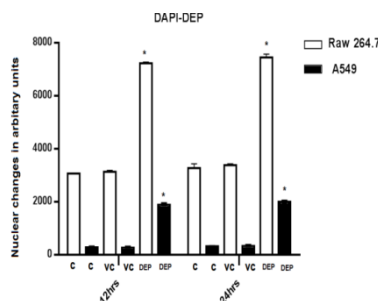
Fig. 3: DNA damage induced by DEPs in human A549 lung cells and RAW264.7 macrophages after 12 and 24 h exposure by measurement of apoptotic levels. Data are expressed as mean±SD of three repeated DEP experiments.* Denotes a significant difference from the control (*p<0.05).
