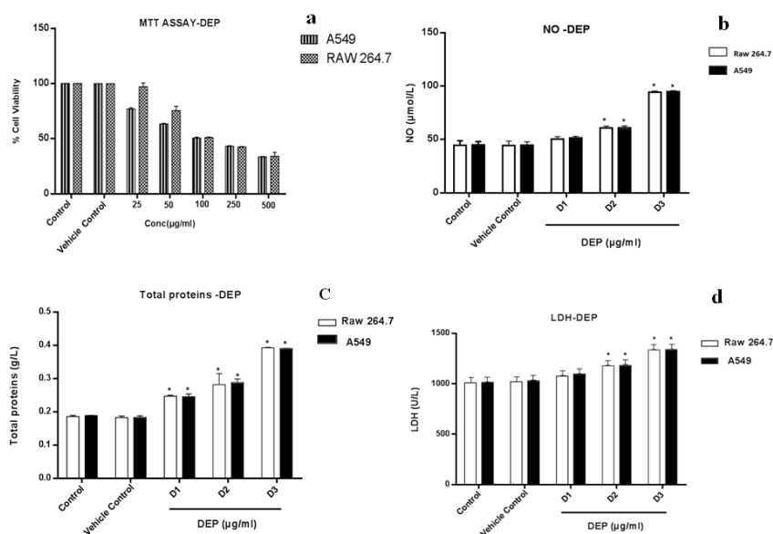
Fig. 1: (a) Cell viability of DEPs exposed to human A549 lung cells and murine RAW 264.7 macrophages after 24 h exposure was determined by MTT assay. Data are expressed as percentage of the control, mean \pm SD of three repeated DEP experiments at the concentration of 25, 50, 100, 250 and 500 \mu\text{g/ml} respectively, (b) Effect of Cytotoxicity of DEPs to human A549 lung cells and murine RAW264.7 macrophages after 24 h exposure by measurement of levels of Nitric oxide (NO), (c) Total Protein (TP) and (d) Lactate dehydrogenase activity (LDH) in culture supernatant fluids. Data are expressed as mean \pm SD of three repeated DEP experiments at different concentrations of DEPs. * Denotes a significant difference from the control (* p < 0.05 ).
