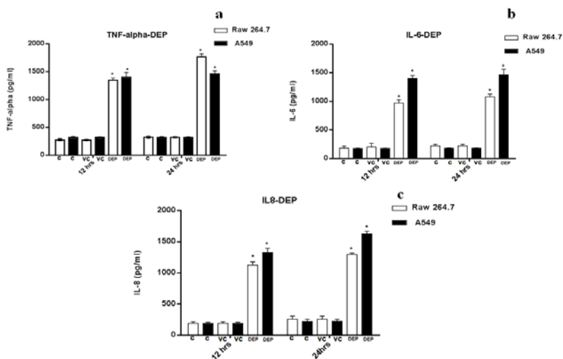
Fig. 4: (a) TNF- \alpha , (b) IL-6 and (c) IL-8 induced by DEPs in human A549 lung cells and RAW264.7 macrophages after 12 and 24 h exposure to DEPs. Data are expressed as mean±SD of three repeated DEPs experiments.* Denotes a significant difference from the control (*p<0.05).
