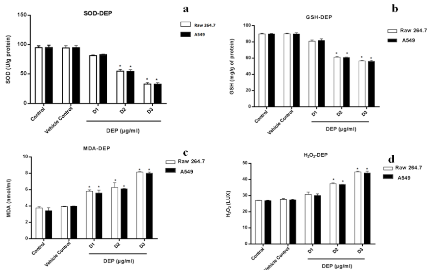
Fig. 2: (a) Oxidative stress induced by DEPs in human A549 lung cells and RAW264.7 macrophages after 24 h exposure by measurement of levels of Superoxide dismutase (SOD), (b) Glutathione (GSH), (c) malondialdehyde (MDA) and (d) hydrogen peroxide (H 2 O 2 ) (after 1h exposure to DEPs), in culture supernatant fluids. Data are expressed as mean±SD of three repeated DEP experiments at different concentrations of DEPs.* Denotes a significant difference from the control (*p<0.05).
