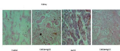
Fig. 3: Histochemical localization of mercury and cadmium in C. batrachus in kidney Control kidney shows no traces of metal. Kidney treated with HgCl 2 exhibits metal deposition in kidney tubules. Kidney exposed to CdSO 4 shows metal accumulation in proximal and distal kidney tubules. Kidney exposed to mixture of Hg + Cd shows less accumulation of metals throughout the kidney section.
